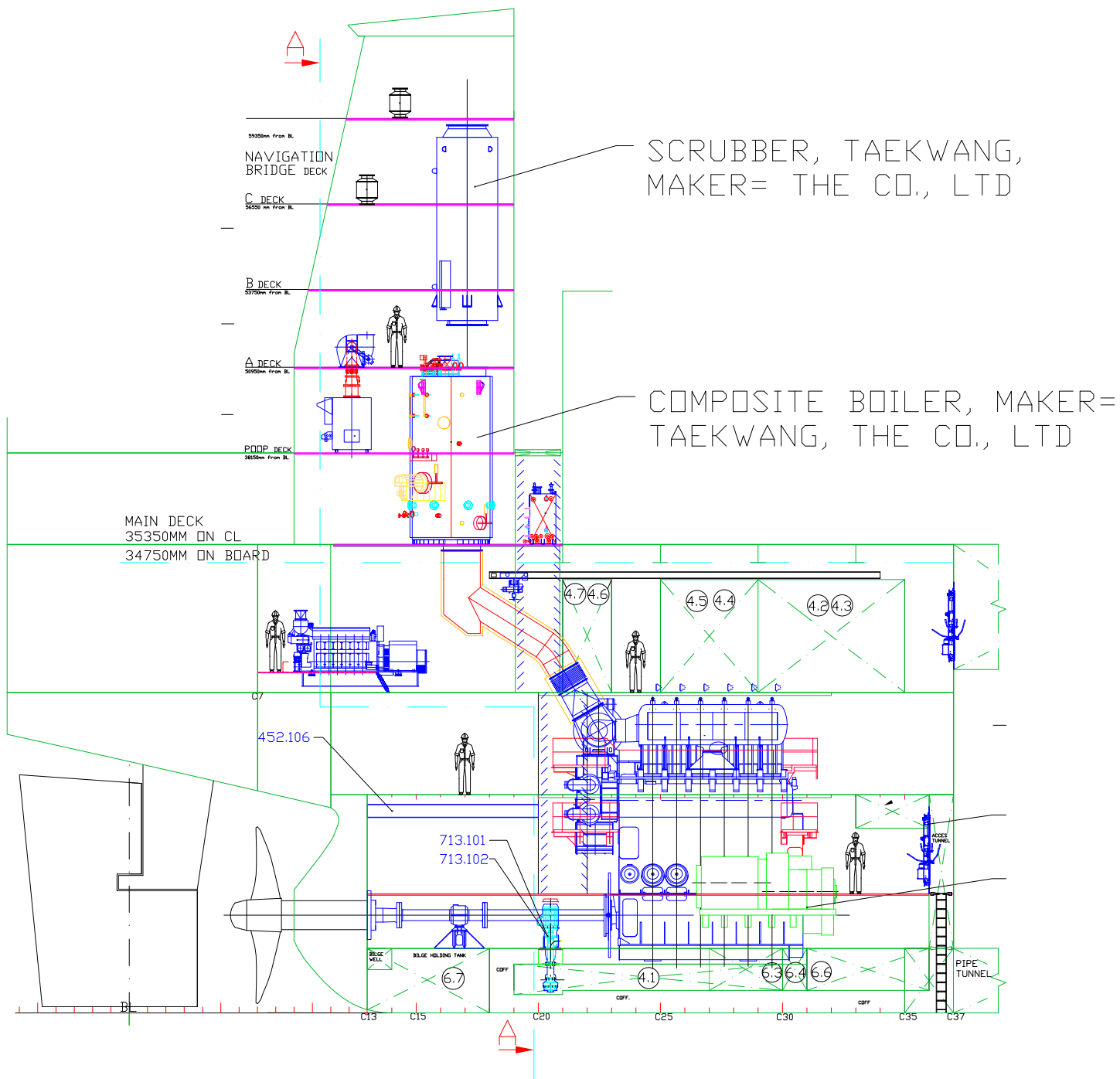
Composite boiler & Scrubber
